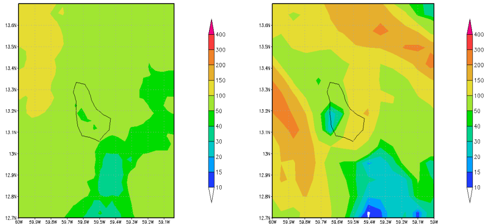
Figure 13 – Accumulated rainfall (in mm) from 1200 UTC on 28 September to 1200 UTC on 29 September over Barbados: satellite-derived (left) and WRF1 (right).
