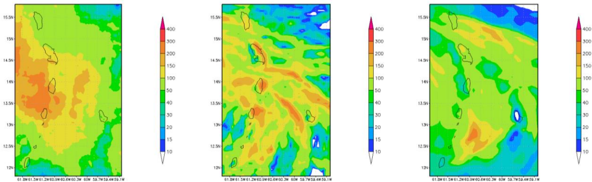
Figure 12 – Accumulated rainfall (in mm) from 1200 UTC on 28 September to 1200 UTC on 29 September over the Windward Islands: satellite-derived (left), WRF1 (centre) and WRF2 (right).
