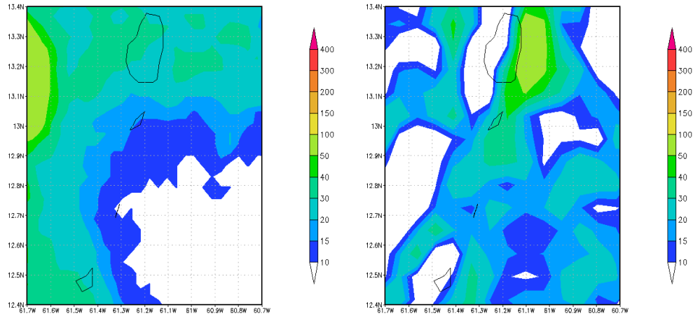
Figure 14 – Accumulated rainfall (in mm) from 1200 UTC on 29 September to 1200 UTC on 30 September over St. Vincent and the Grenadines: satellite-derived (left) and WRF1 (right).
