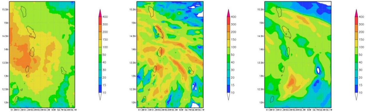
Figure 12 – Accumulated rainfall (in mm) from 12 UTC of 28 September to 12 UTC of 29 September over Windward Islands: satellite-derived (left), WRF1 (center) and WRF2 (right).
