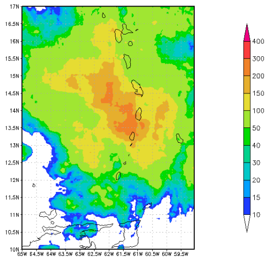
Figure 11 – Satellite derived accumulated rainfall (in mm) from 12 UTC of 28 September to 12 UTC of 30 September over Windward Islands.
