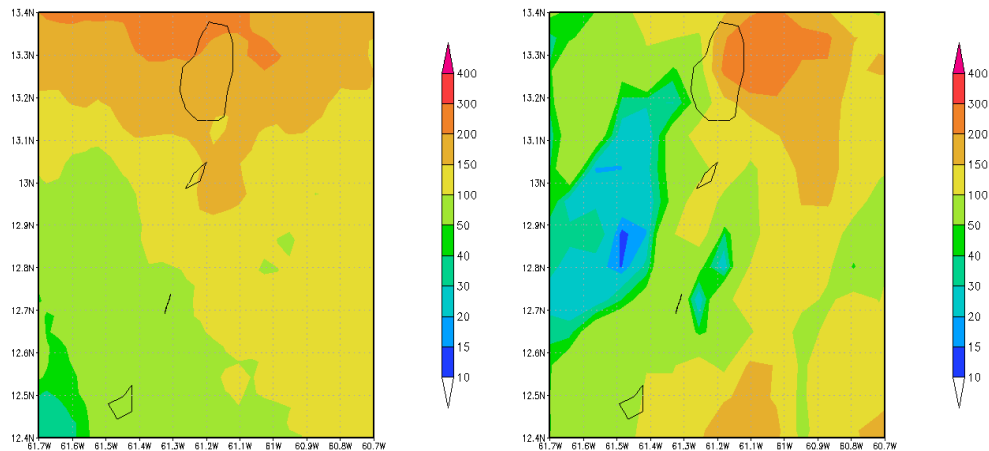
Figure 13 – Accumulated rainfall (in mm) from 1200 UTC on 28 September to 1200 UTC on 30 September over St. Vincent and the Grenadines: satellite-derived (left) and WRF1 (right).
