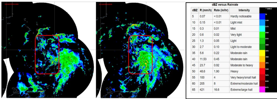
Figure 3 – Reflectivity maps of Caribbean radar composite (source: http://barbadosweather.org/Composite/ ) centred over Lesser Antilles at 15:00 UTC (left) and 18:00 UTC (centre) reflectivity relationship table (right).
