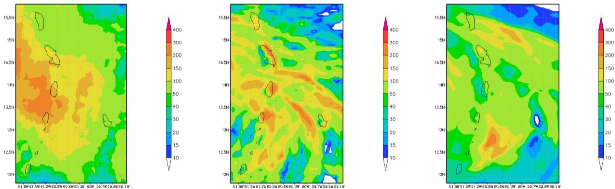
Figure 11 – Accumulated rainfall (in mm) from 12 UTC of 28 September to 12 UTC of 29 September over Windward Islands: satellite-derived (left), WRF1 (center) and WRF2 (right).
