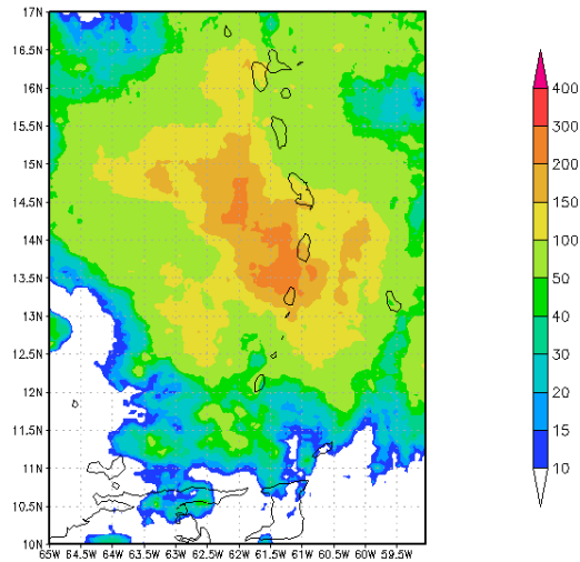
Figure 10 – Satellite derived accumulated rainfall (in mm) from 12 UTC of 28 September to 12 UTC of 29 September over Windward Islands.
