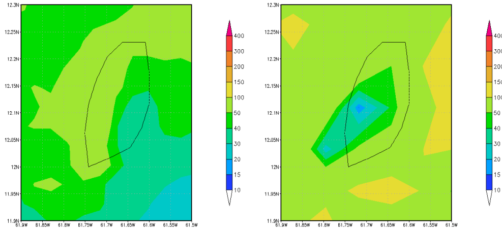
Figure 12 – Accumulated rainfall (in mm) from 12 UTC of on 28 September to 1200 UTC on 29 September over Grenada: satellite-derived (left) and WRF1 (right).
