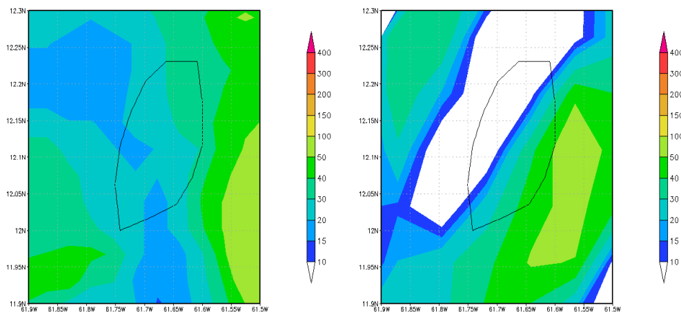
Figure 13 – Accumulated rainfall (in mm) from 1200 UTC on 29 September to 1200 UTC on 30 September over Grenada: satellite-derived (left) and WRF1 (right).
