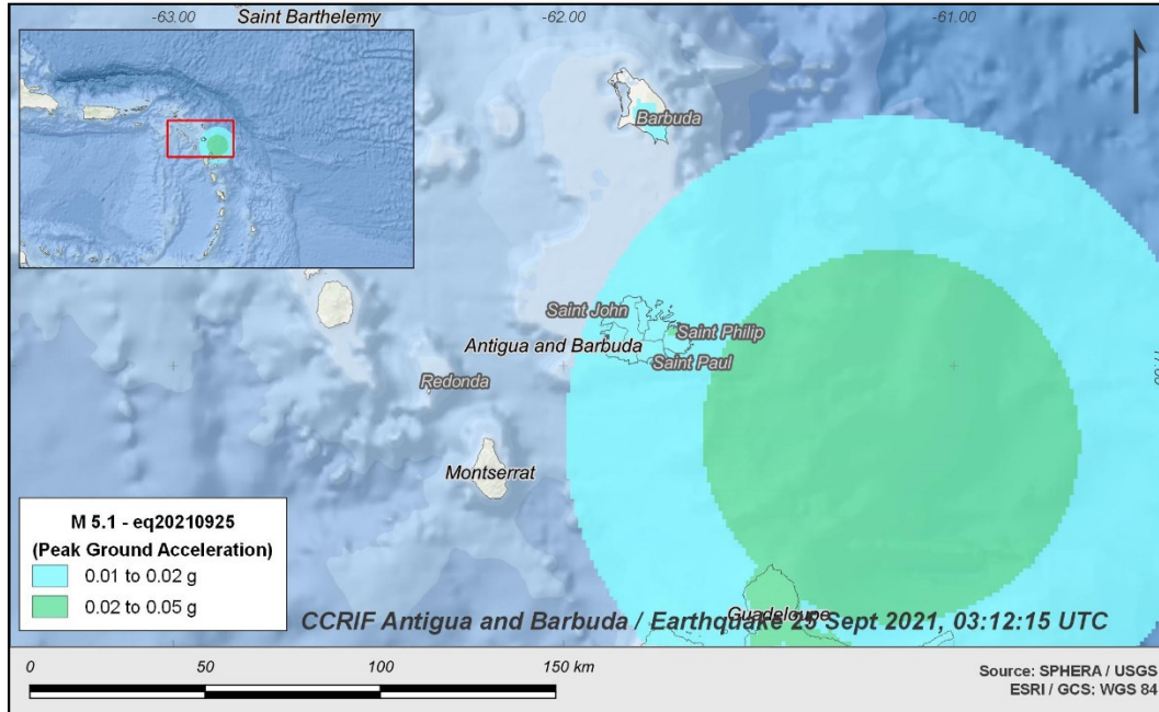
Figure 2 Map showing the peak ground acceleration in Antigua and Barbuda computed using SPHERA model following the magnitude 5.1 earthquake on 25 September at 03:12:15 UTC. Source: USGS & CCRIF SPHERA EQ Model.
