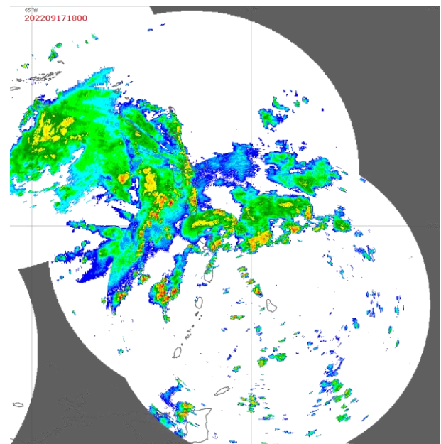
d) 17 September at 1800 UTC
