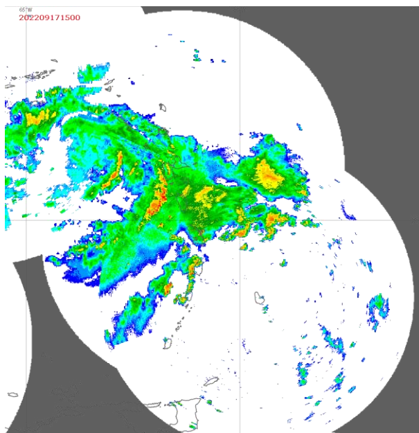
c) 17 September at 1500 UTC
