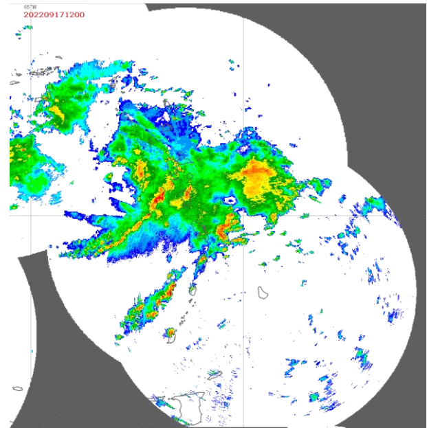
b) 17 September at 1200 UTC
