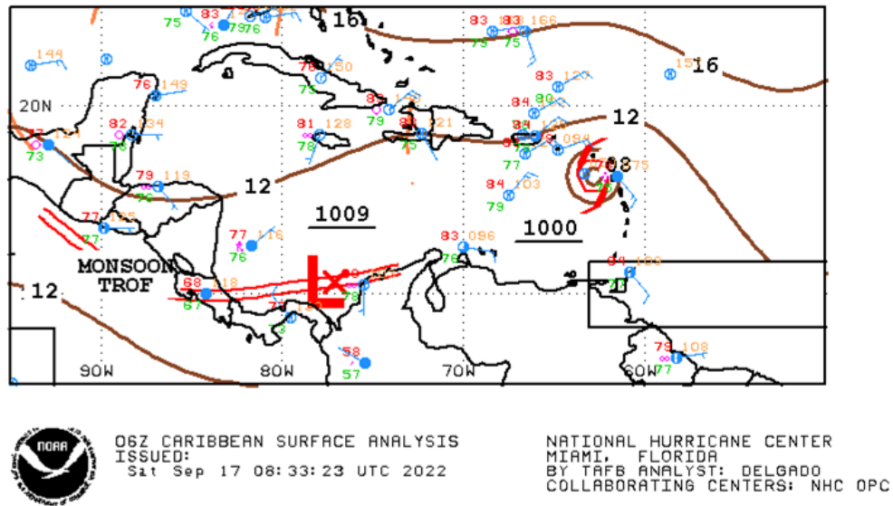
Figure 1 Surface analysis over the Caribbean area on 17 September at 0600UTC. Tropical Cyclone Fiona was located over the Northern Leeward Islands. Source: US National Hurricane Center 1
