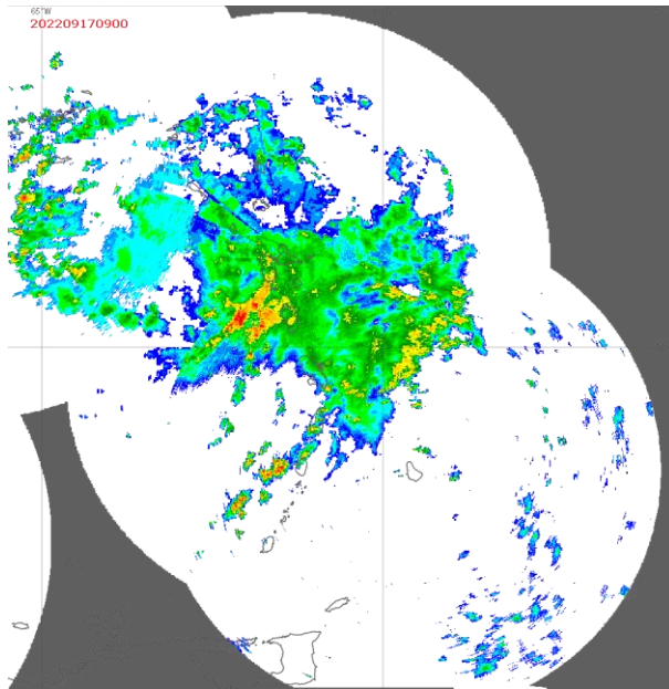
a) 17 September at 0900 UTC
