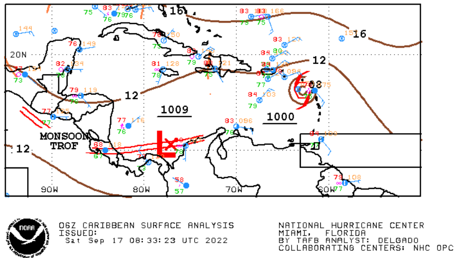
Figure 1 Surface analysis over the Caribbean area on 17 September 2022 at 0600UTC. Tropical Cyclone Fiona was located over the northern Leeward Islands. Source: US National Hurricane Center 1
