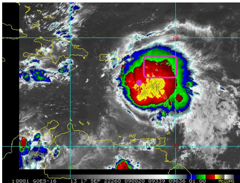
Figure 2 Satellite imagery on 17 September 2022 at 0900UTC from thermal infrared channel enhanced with colour. Blue/green colours represent high altitude clouds (top cloud temperature between -50^{\circ}\text{C} and -70^{\circ}\text{C} ), while the red/yellow colours represent very high altitude clouds (top cloud lower than -70^{\circ}\text{C} ). High altitude clouds indicate strong convection associated with intense precipitation. The circulation centre is indicated by the violet point, while the Northern Leeward Islands are surrounded by a violet square. Source: NOAA, National Environmental Satellite, Data and Information Service 2 .
