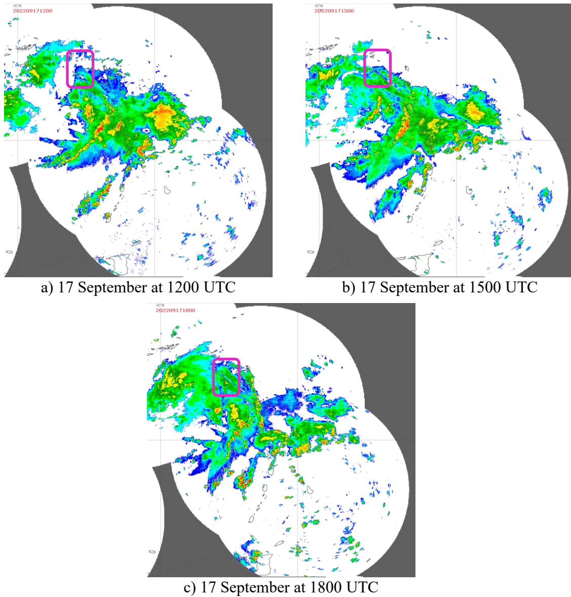
Figure 3 Radar imagery on 17 September at 1200 UTC (a) at 1500 UTC (b) and at 1800 UTC (c) as indicated in the label from the radar composite over the Caribbean and Central America region. Blue/green colours represent low to moderate rainfall, while the yellow/red colours represent intense and very intense precipitation. The violet square highlights the location of Saint Kitts and Nevis. Source: Barbados Radar Composite 3 .
