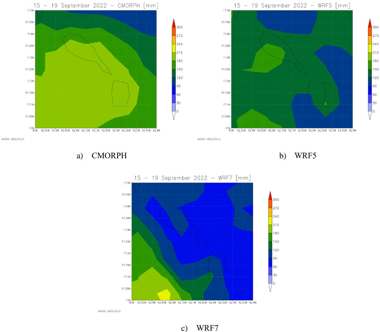
Figure 5 Total accumulated precipitation during the period 15-19 September, 2022 estimated by CMORPH (a), WRF5 (b) and WRF7 (c). Source: CCRIF SPC
