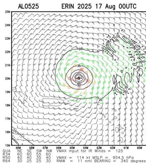
c) 17 August at 0000UTC
