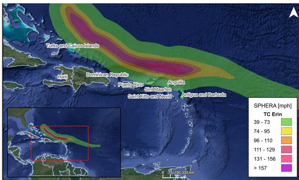
Figure 4 Map showing the wind field associated with Tropical Cyclone Erin around the Leeward Islands.
