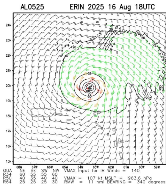
b) 16 August at 1800UTC
