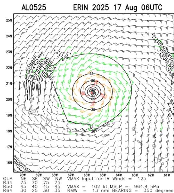
c) 17 August at 0600UTC
