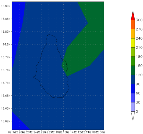
08 OCT – 10 OCT 2025 – IMERG7 [mm]
