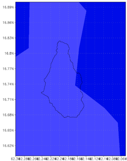
08 OCT – 10 OCT 2025 – CMORPH [mm]
