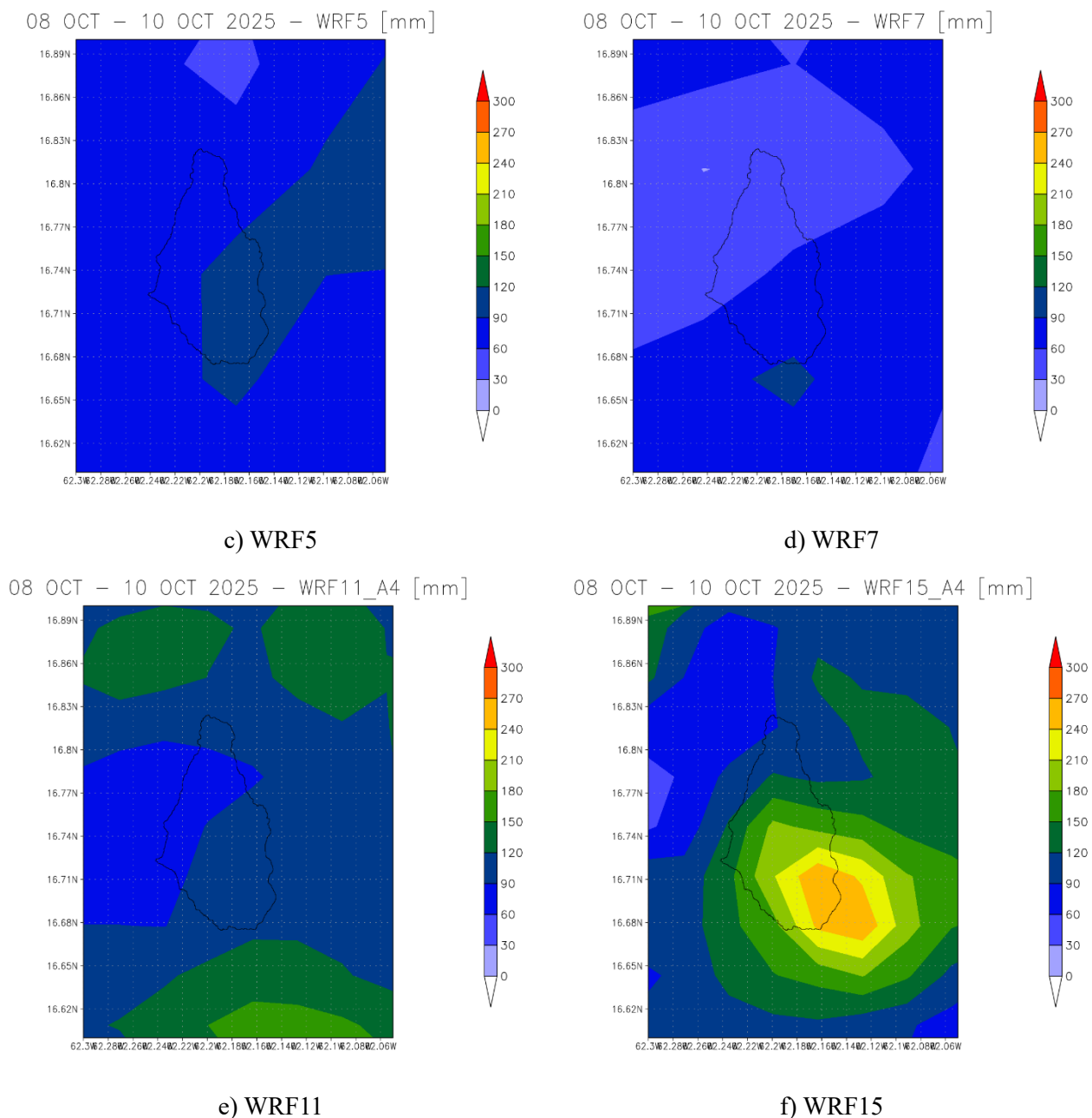
Figure 4 Total accumulated precipitation during the period 08 to 10 October 2025 estimated by CMORPH (a), IMERG7 (b), WRF5 (c), WRF7 (d), WRF11 (e), WRF15 (f). Source: CCRIF SPC
